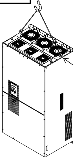
Eye bolt
