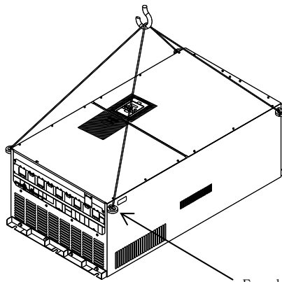
Eye bolt
